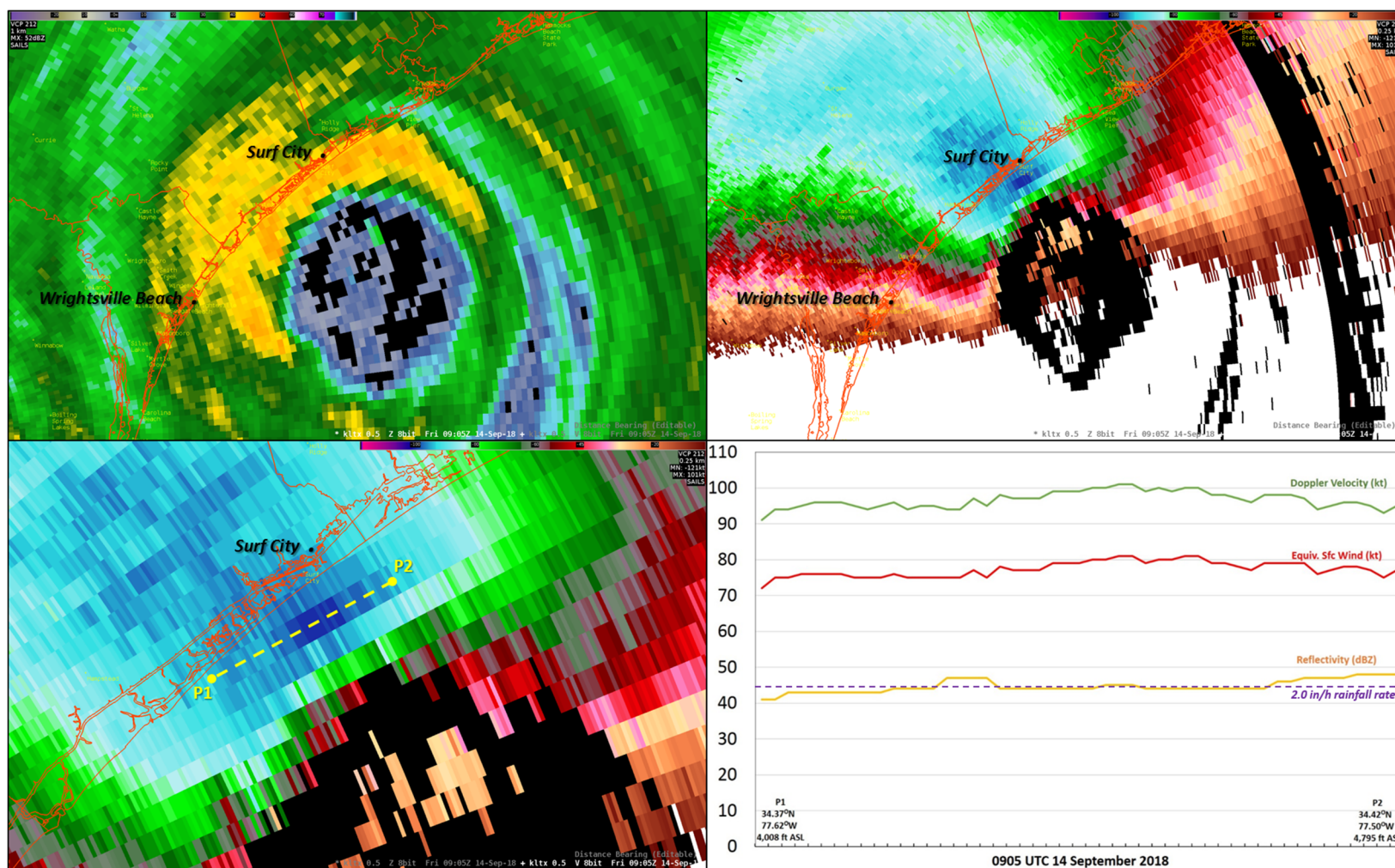
Figure 7. Wilmington, North Carolina (KLTX) WSR-88D Doppler weather radar view of Florence's large eye at 0905 UTC 14 September about 2 h prior to landfall; antenna elevation was 0.5° — (a) Reflectivity (dBZ), (b) Doppler velocity (kt), (c) zoomed-in Doppler velocity (250-meter intervals) along the 060° azimuthal radial (relative to KLTX), and (d) analysis along the radial from endpoints P1 to P2: Doppler Velocity (kt; green line), Equivalent Surface Wind Speed (kt; red line), Reflectivity (dBZ; orange line; 2.0 in/h rainfall rate (dashed purple line).
